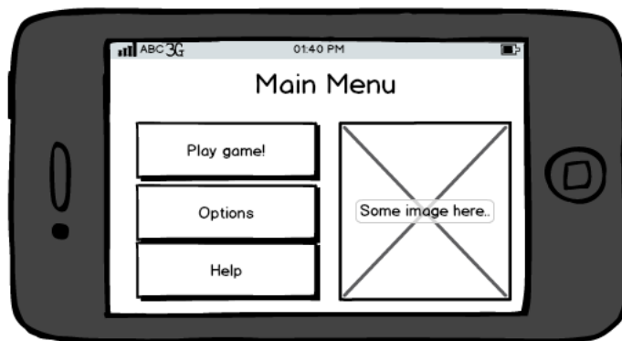
Figure 7: Main menu.
